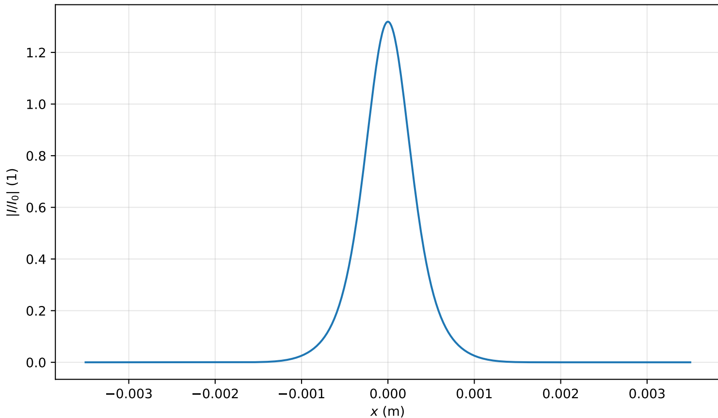
Intensity profile I(x, y = 0, z = 1.115m)/I_0 , P_{in}=0.8P_{cr} , artificial time
